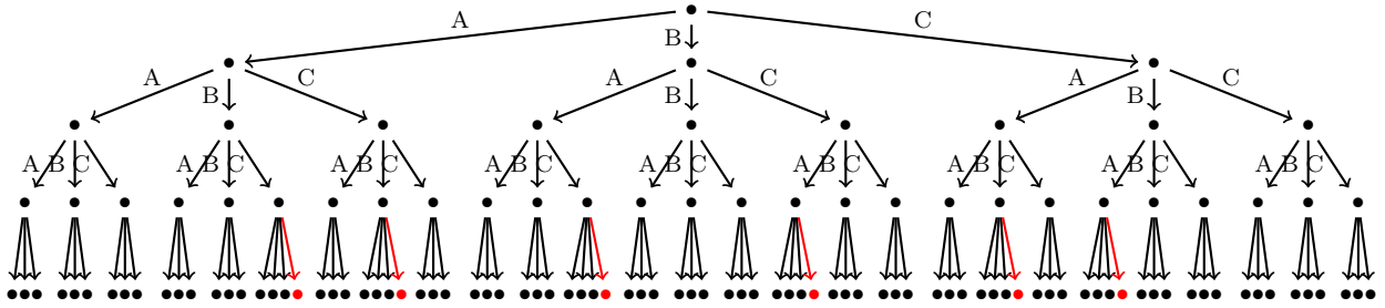
Fig. 2 The search tree of our running example, where the missed labels of edges in black color are respectively A,B,C, and the missed labels of edges in red color are Submit
