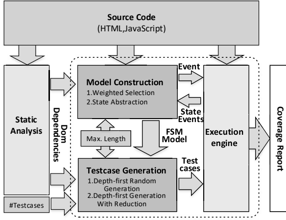
Fig. 3 Framework overview of LJS
