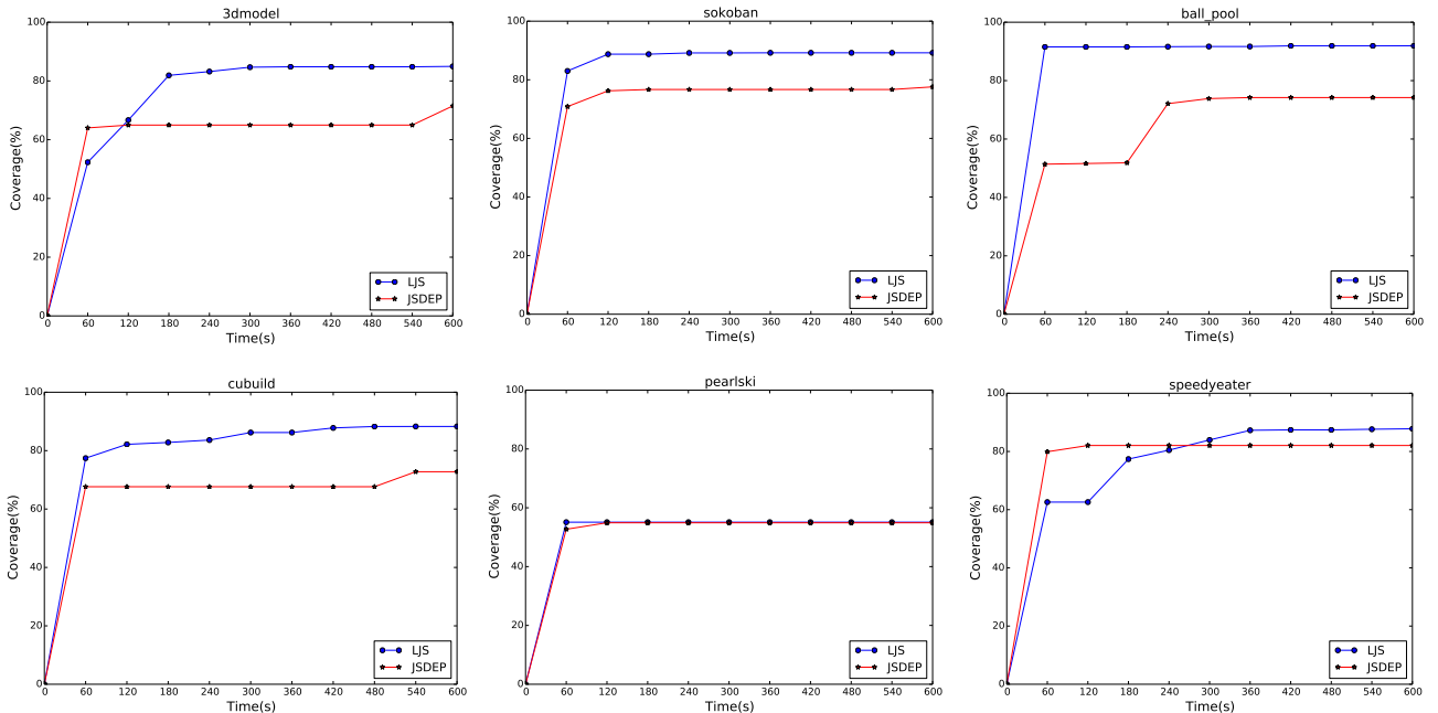
Fig. 5 Coverage of LJS and JSDEP, as a function of the execution time
